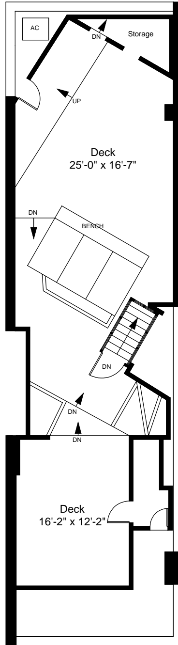
Roof Plan
